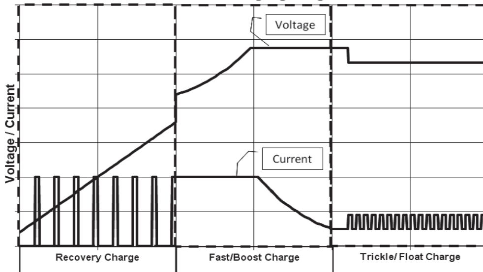
CB Charging Diagram
