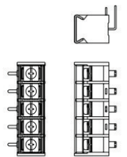
90 deg. terminal optional with plastic cover (has MOQ required)
